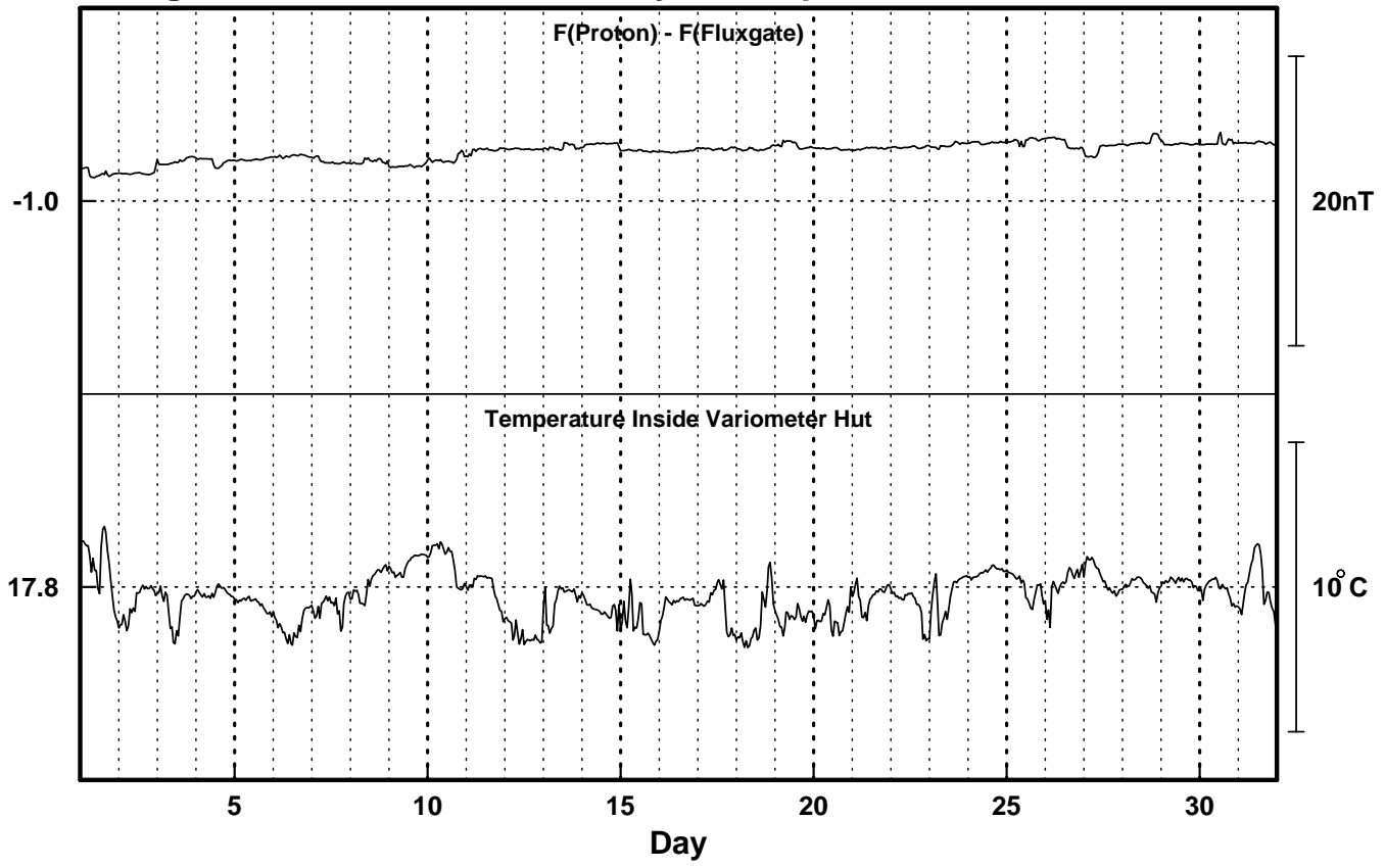
Figure 2 : Sable Island Monthly F Comparison December 2000
