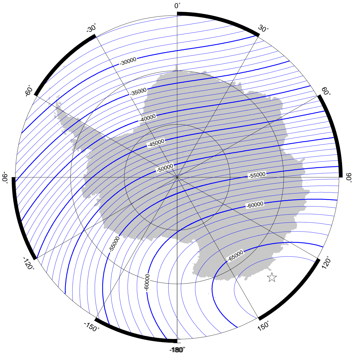
Vertical component ( Z ) in region of south pole at 2015.0 from the World Magnetic Model (WMM2015v2). Contour interval is 1000 nT, white star is location of a magnetic pole and projection is Polar Stereographic. Credit: British Geological Survey (UK Research and Innovation).
