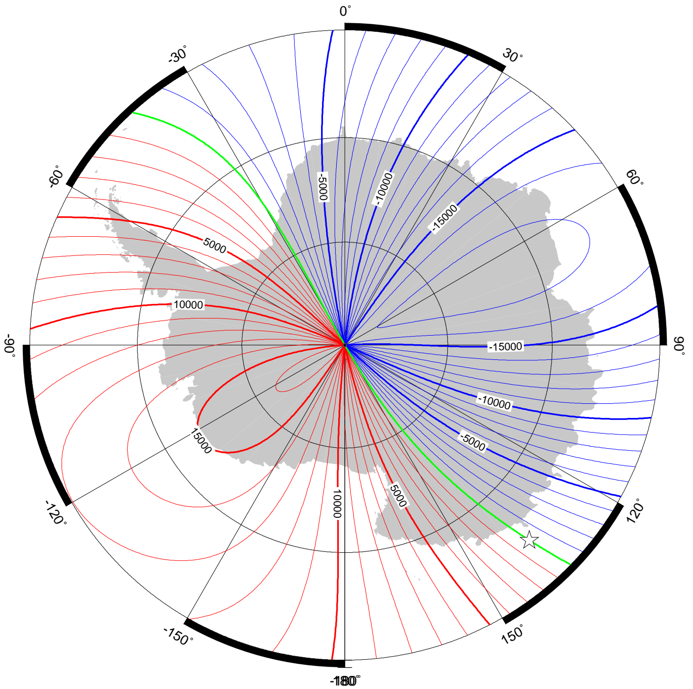
East component (Y) in region of south pole at 2015.0 from the World Magnetic Model (WMM2015v2). Red - positive (east), blue - negative (west), green - zero. Contour interval is 1000 nT, white star is location of a magnetic pole and projection is Polar Stereographic. Credit: British Geological Survey (UK Research and Innovation).
