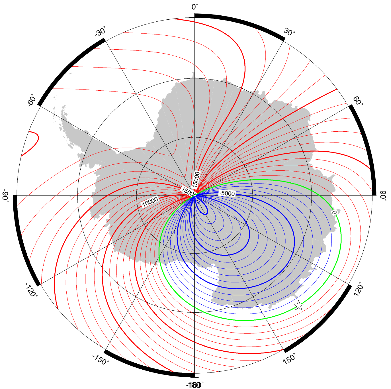
North component ( X ) in region of south pole at 2015.0 from the World Magnetic Model (WMM2015v2). Red - positive (north), blue - negative (south), green - zero. Contour interval is 1000 nT, white star is location of a magnetic pole and projection is Polar Stereographic. Credit: British Geological Survey (UK Research and Innovation).
