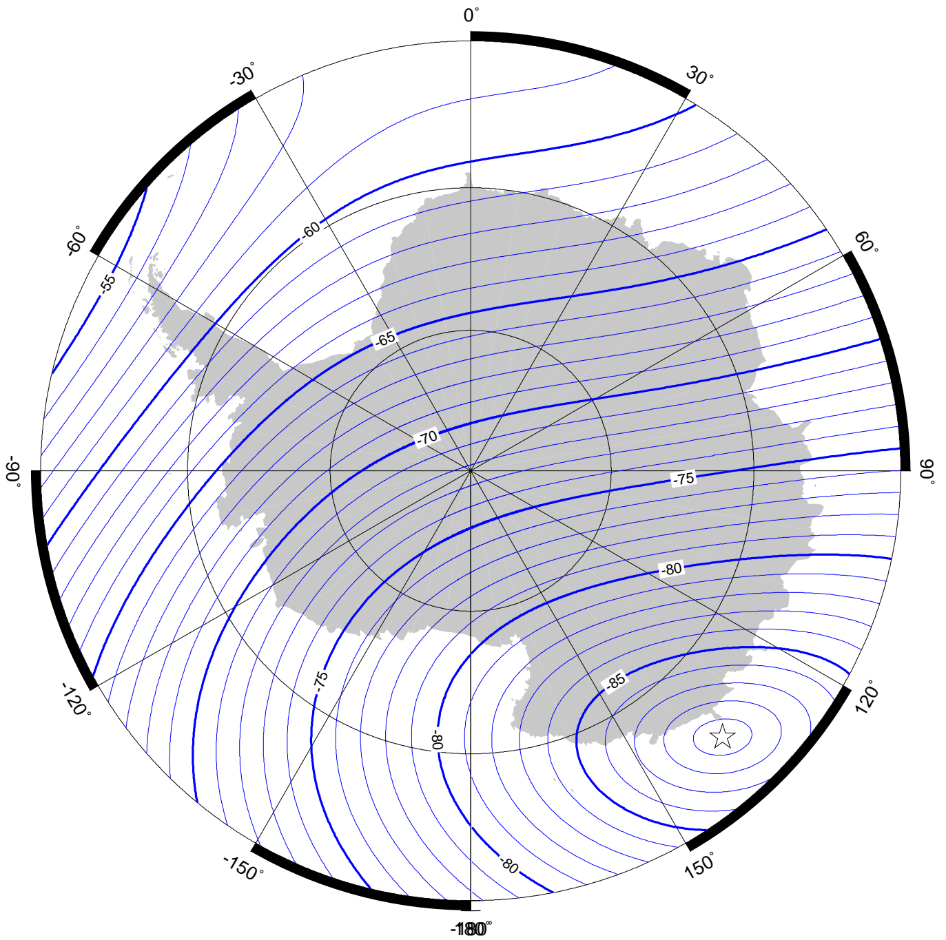
Inclination (magnetic dip) in region of south pole at 2015.0 from the World Magnetic Model (WMM2015v2). Contour interval is 1^\circ , white star is location of a magnetic pole and projection is Polar Stereographic. Credit: British Geological Survey (UK Research and Innovation).
