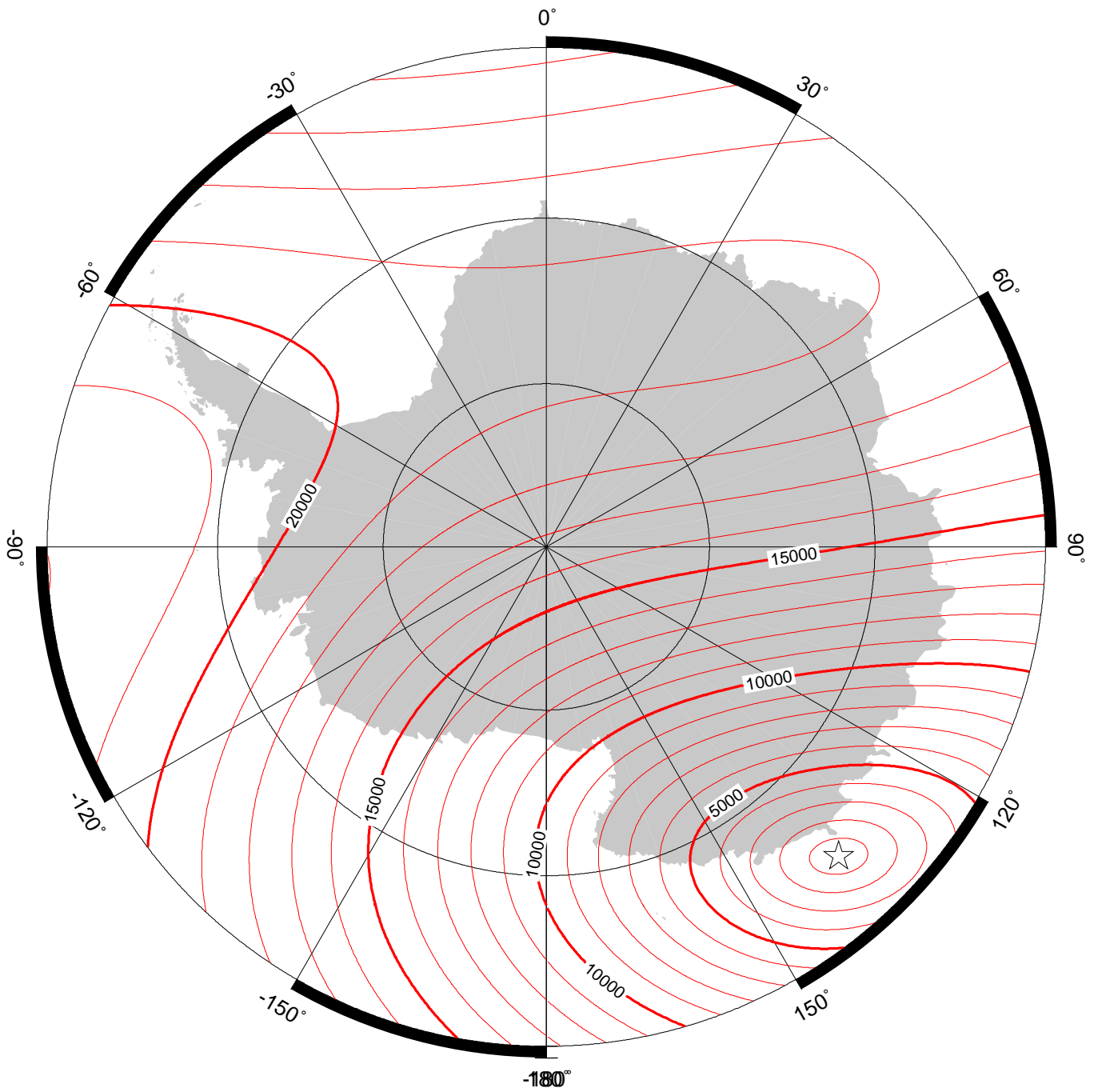
Horizontal intensity ( H ) in region of south pole at 2015.0 from the World Magnetic Model (WMM2015v2). Contour interval is 1000 nT, white star is location of a magnetic pole and projection is Polar Stereographic. Credit: British Geological Survey (UK Research and Innovation).
