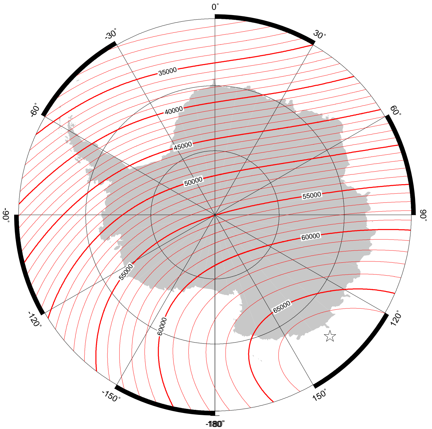
Total intensity ( F ) in region of south pole at 2015.0 from the World Magnetic Model (WMM2015v2). Contour interval is 1000 nT, white star is location of a magnetic pole and projection is Polar Stereographic. Credit: British Geological Survey (UK Research and Innovation).
