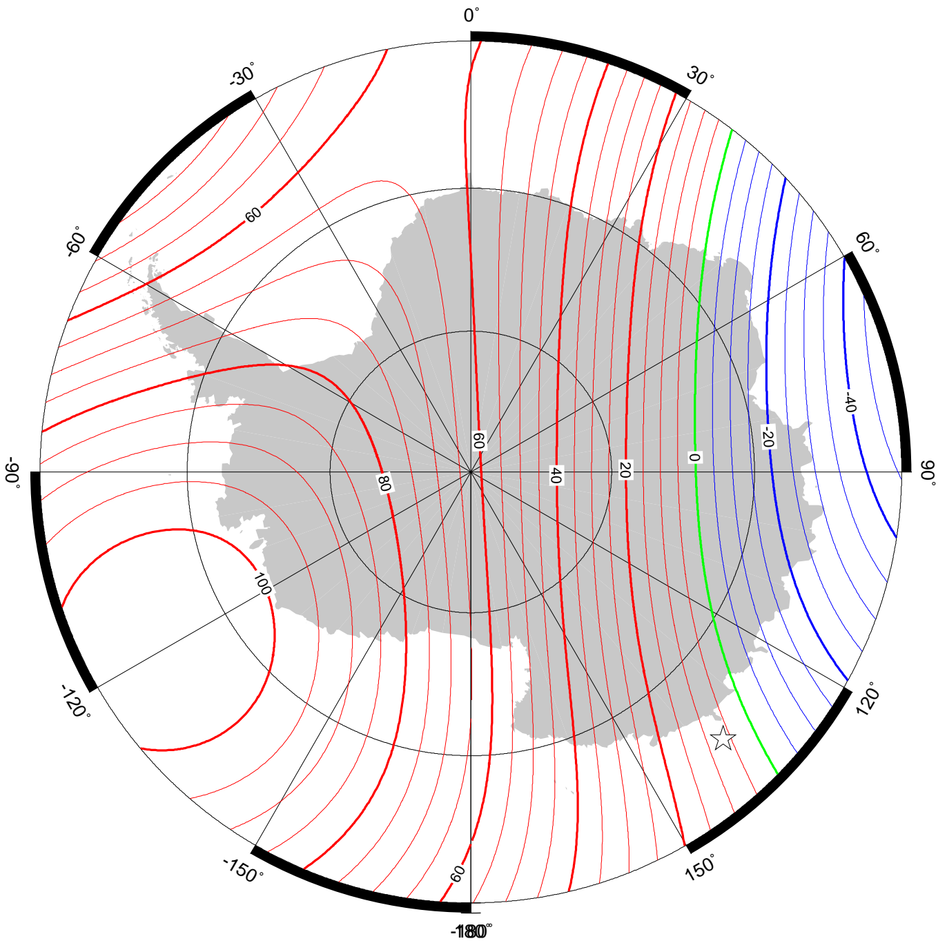
Annual rate of change of vertical component in region of south pole for 2015.0 to 2020.0 from the World Magnetic Model (WMM2015v2). Red - positive change, blue - negative change, green - zero change. Contour interval is 5 nT/year, white star is location of a magnetic pole and projection is Polar Stereographic. Credit: British Geological Survey (UK Research and Innovation).
