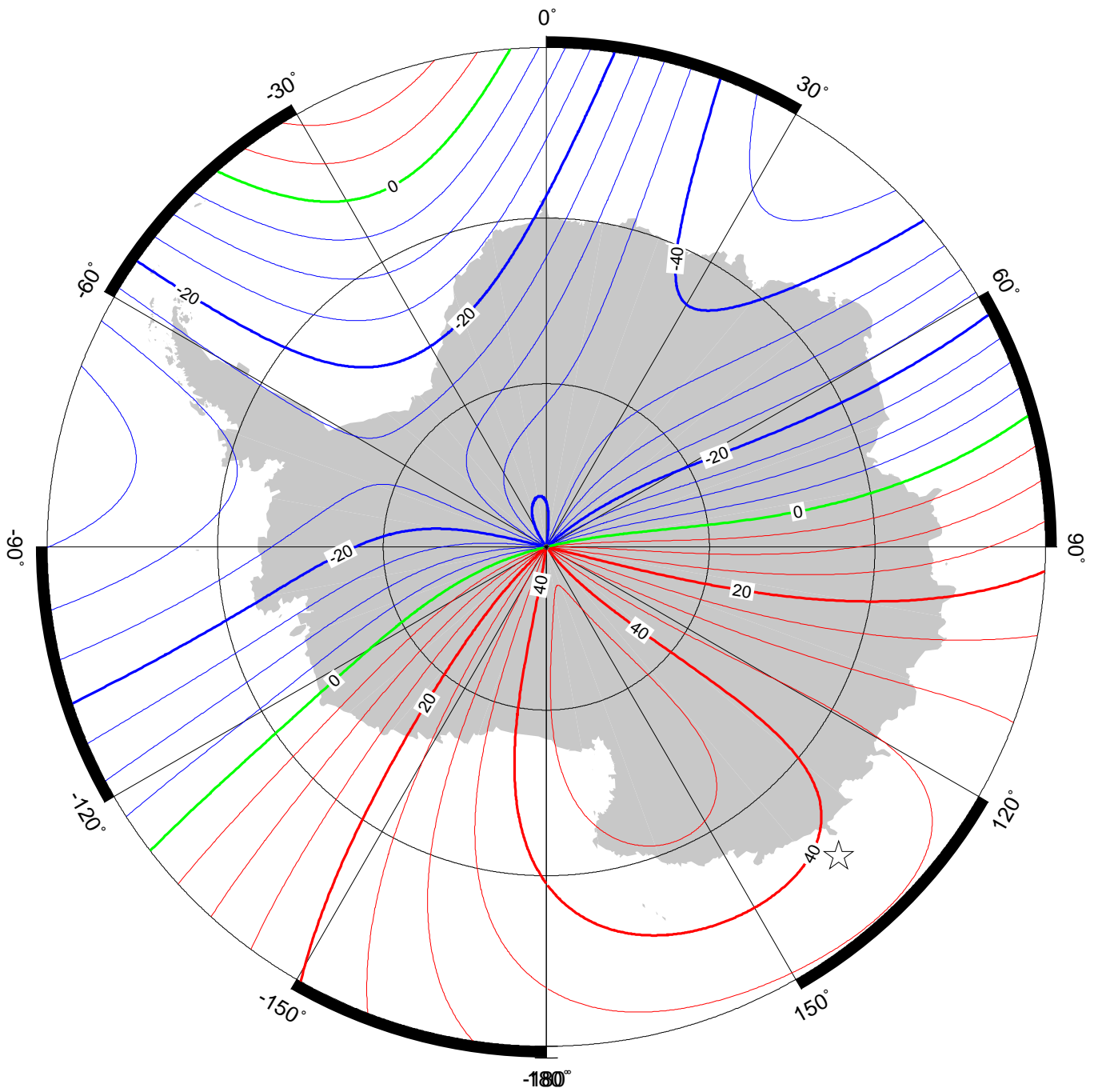
Annual rate of change of east component in region of south pole for 2015.0 to 2020.0 from the World Magnetic Model (WMM2015v2). Red - positive change, blue - negative change, green - zero change. Contour interval is 5 nT/year, white star is location of a magnetic pole and projection is Polar Stereographic. Credit: British Geological Survey (UK Research and Innovation).
