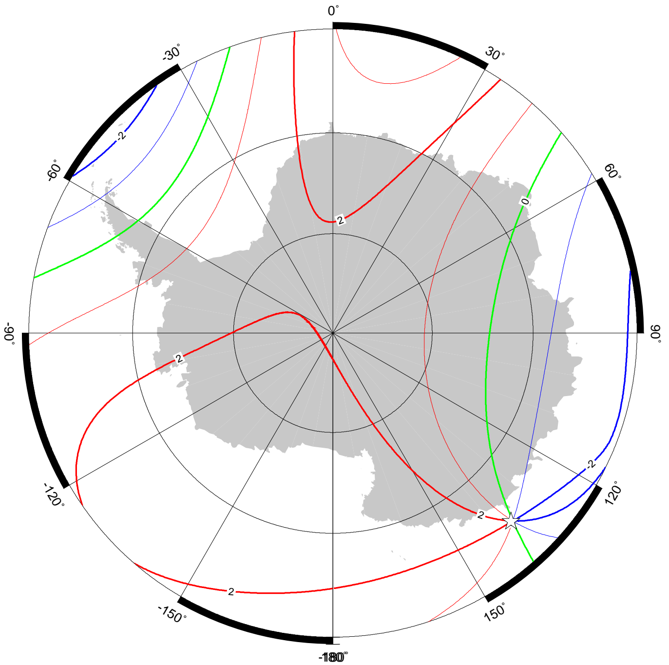
Annual rate of change of inclination in region of south pole for 2015.0 to 2020.0 from the World Magnetic Model (WMM2015v2). Red - positive change, blue - negative change, green - zero change. Contour interval is 1°/year, white star is location of a magnetic pole and projection is Polar Stereographic. Credit: British Geological Survey (UK Research and Innovation).
