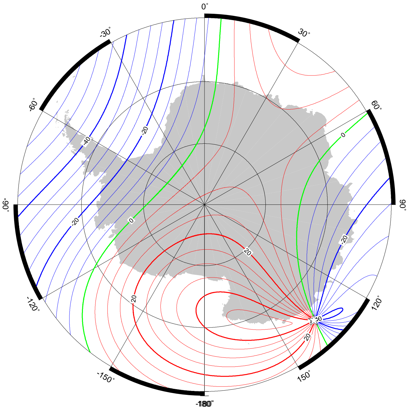
Annual rate of change of horizontal intensity in region of south pole for 2015.0 to 2020.0 from the World Magnetic Model (WMM2015v2). Red - positive change, blue - negative change, green - zero change. Contour interval is 5 nT/year, white star is location of a magnetic pole and projection is Polar Stereographic. Credit: British Geological Survey (UK Research and Innovation).
