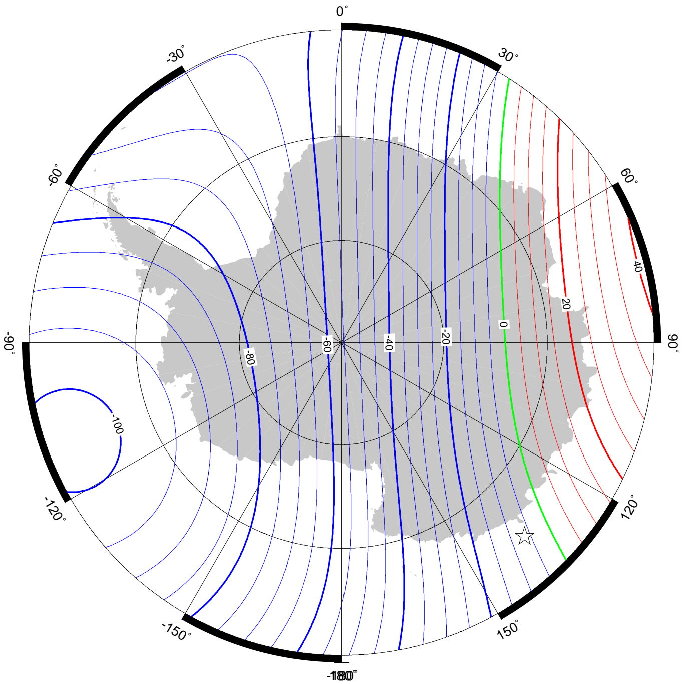
Annual rate of change of total intensity in region of south pole for 2015.0 to 2020.0 from the World Magnetic Model (WMM2015v2). Red - positive change, blue - negative change, green - zero change. Contour interval is 5 nT/year, white star is location of a magnetic pole and projection is Polar Stereographic. Credit: British Geological Survey (UK Research and Innovation).
