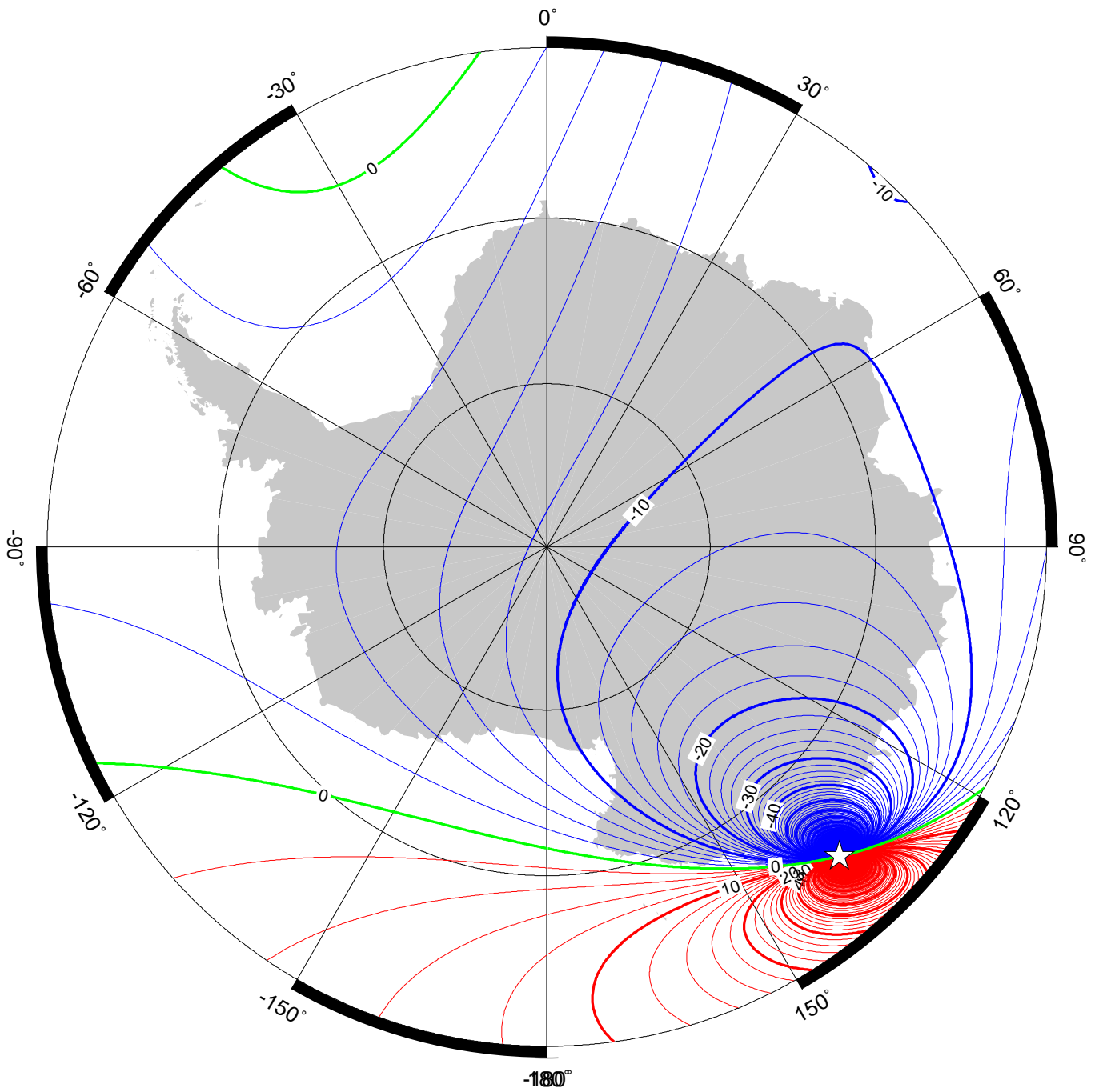
Annual rate of change of declination in region of south pole for 2015.0 to 2020.0 from the World Magnetic Model (WMM2015v2). Red - easterly change, blue - westerly change, green - zero change. Contour interval is 2°/year, white star is location of a magnetic pole and projection is Polar Stereographic. Credit: British Geological Survey (UK Research and Innovation).
