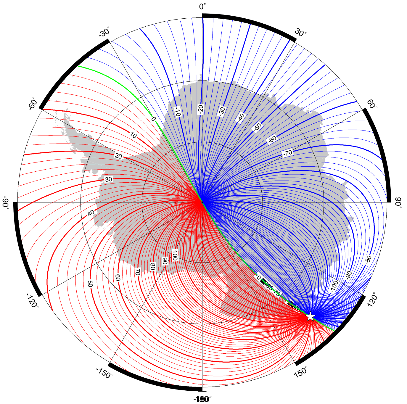
Declination (magnetic variation) in region of south pole at 2015.0 from the World Magnetic Model (WMM2015v2). Red - positive (east), blue - negative (west), green - zero. Contour interval is 2°, white star is location of a magnetic pole and projection is Polar Stereographic. Credit: British Geological Survey (UK Research and Innovation).
