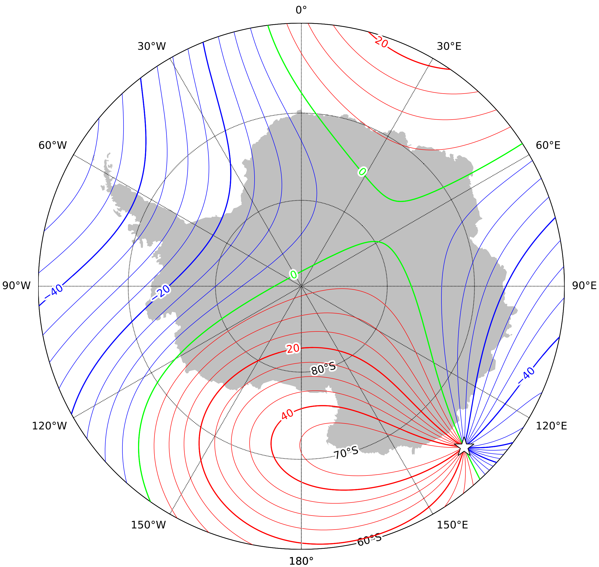
Annual rate of change of horizontal intensity in the region of the south pole at 2027.5 from the World Magnetic Model (WMM) 2025. Red - positive change, blue - negative change, green - zero change. Contour interval is 5nT/year, white star is the location of a magnetic pole and the projection is Polar Stereographic. This is an example of an isoporic chart.
