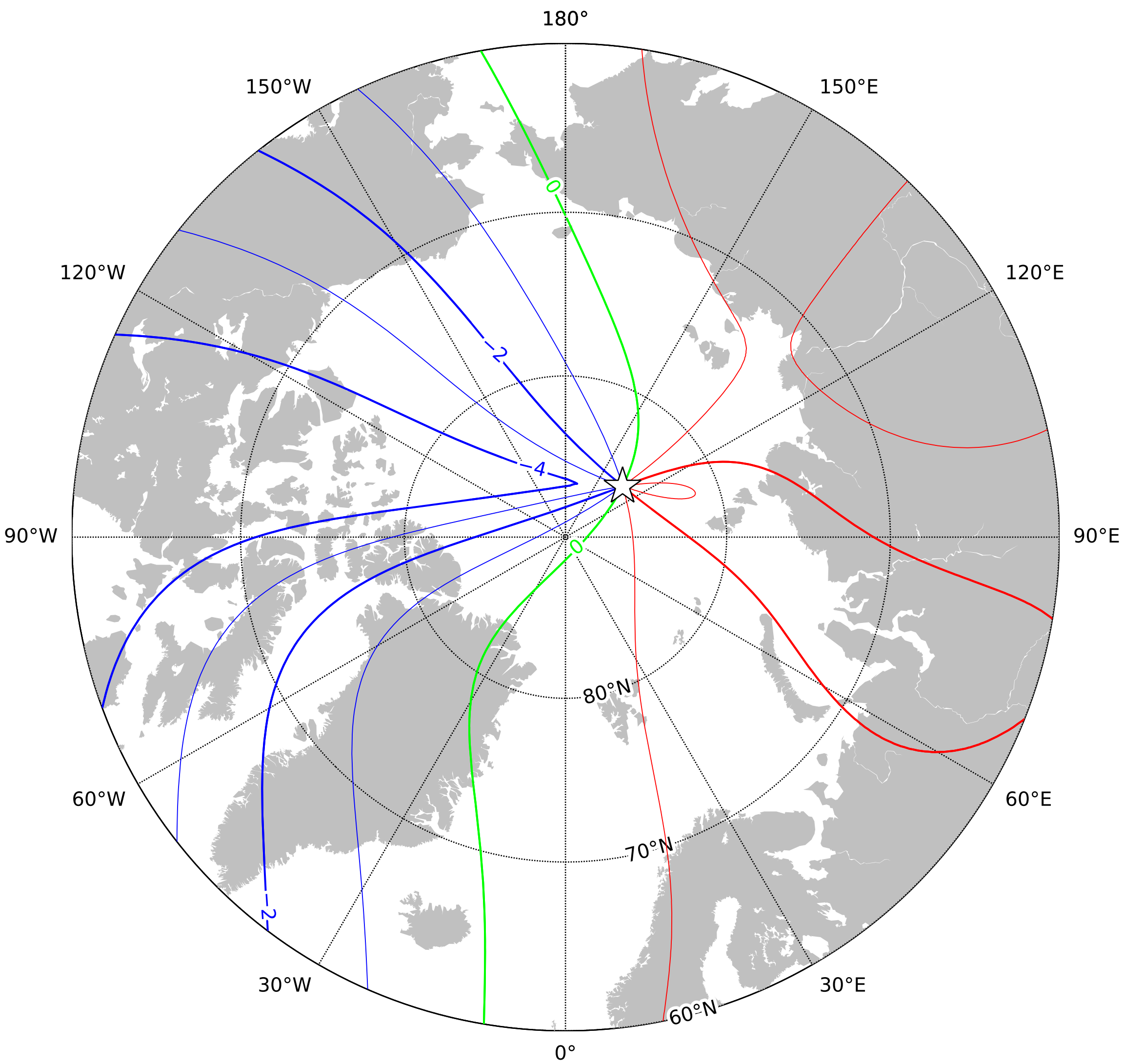
Annual rate of change of inclination in the region of the north pole at 2027.5 from the World Magnetic Model (WMM) 2025. Red - positive (downward) change, blue - negative (upward) change, green - zero change. Contour interval is 1'/year, white star is the location of a magnetic pole and the projection is Polar Stereographic. This is an example of an isoporic chart. British Geological Survey © UKRI 2024
