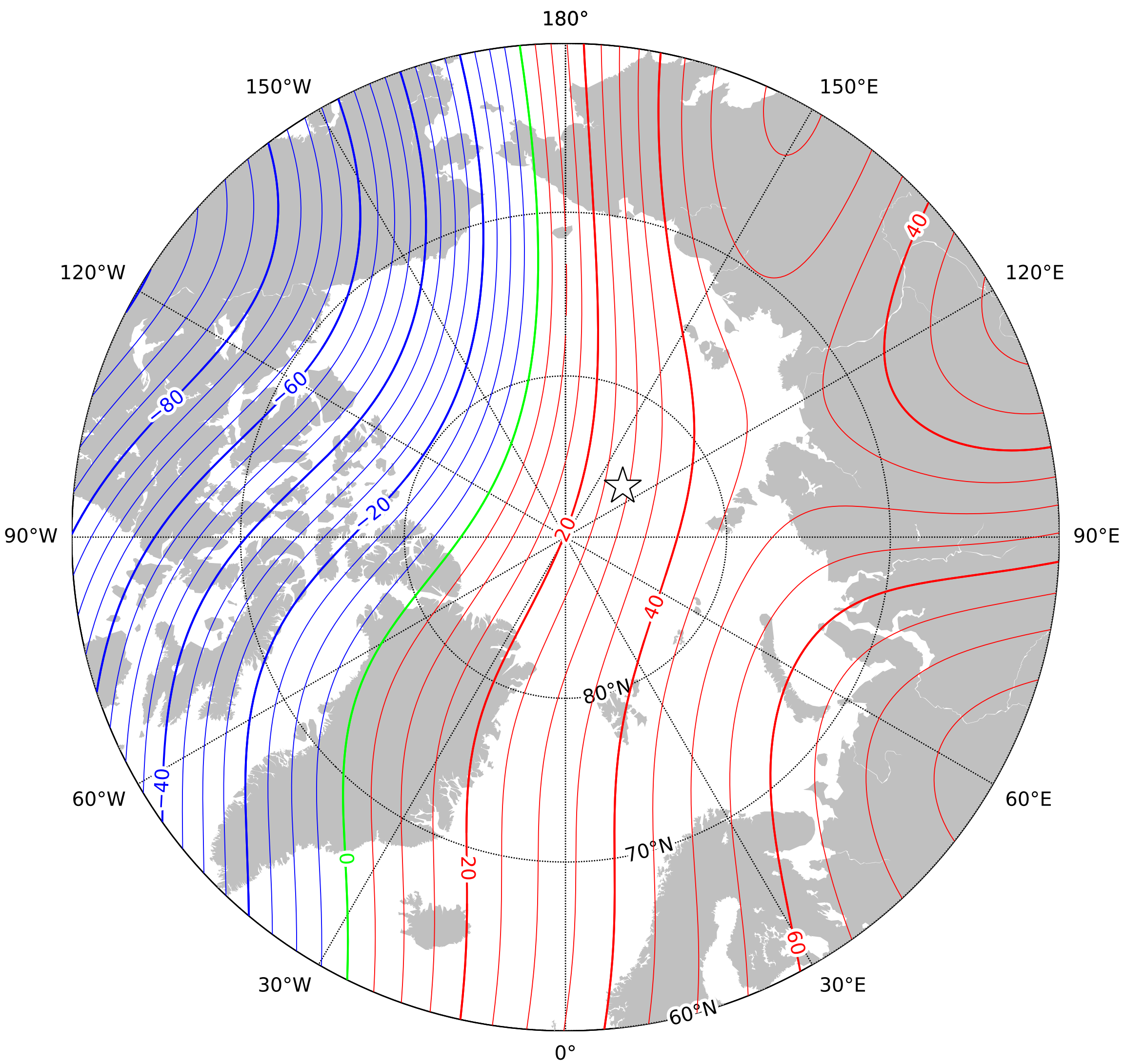
Annual rate of change of downward component in the region of the north pole at 2027.5 from the World Magnetic Model - High Resolution (WMMHR) 2025 (core component only). Red - positive (downward) change, blue - negative (upward) change, green - zero change. Contour interval is 5nT/year, white star is the location of a magnetic pole and the projection is Polar Stereographic. This is an example of an isoporic chart. British Geological Survey © UKRI 2024
