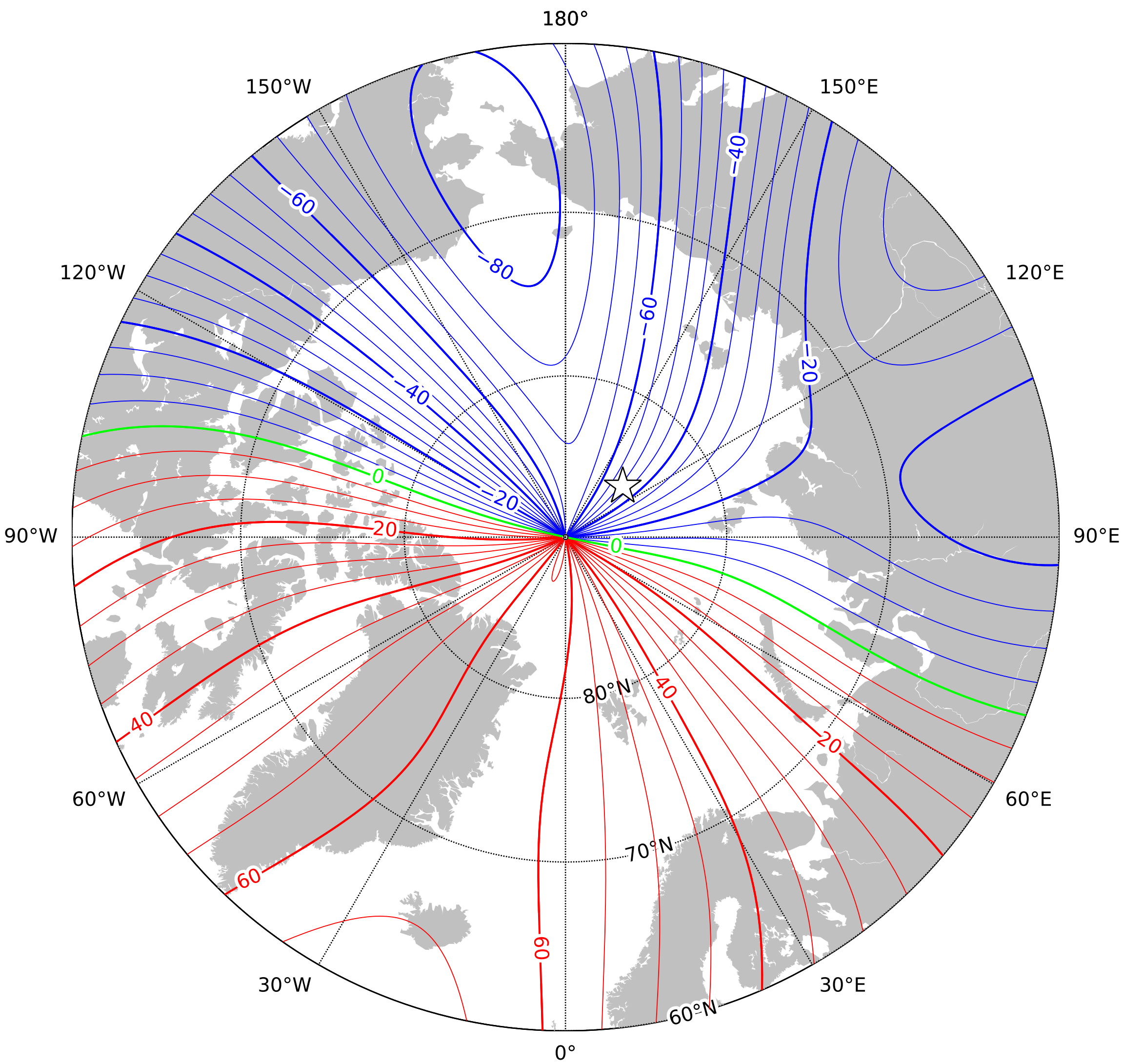
Annual rate of change of east component in the region of the north pole at 2027.5 from the World Magnetic Model - High Resolution (WMMHR) 2025 (core component only). Red - positive (easterly) change, blue - negative (westerly) change, green - zero change. Contour interval is 5nT/year, white star is the location of a magnetic pole and the projection is Polar Stereographic. This is an example of an isoporic chart. British Geological Survey © UKRI 2024
