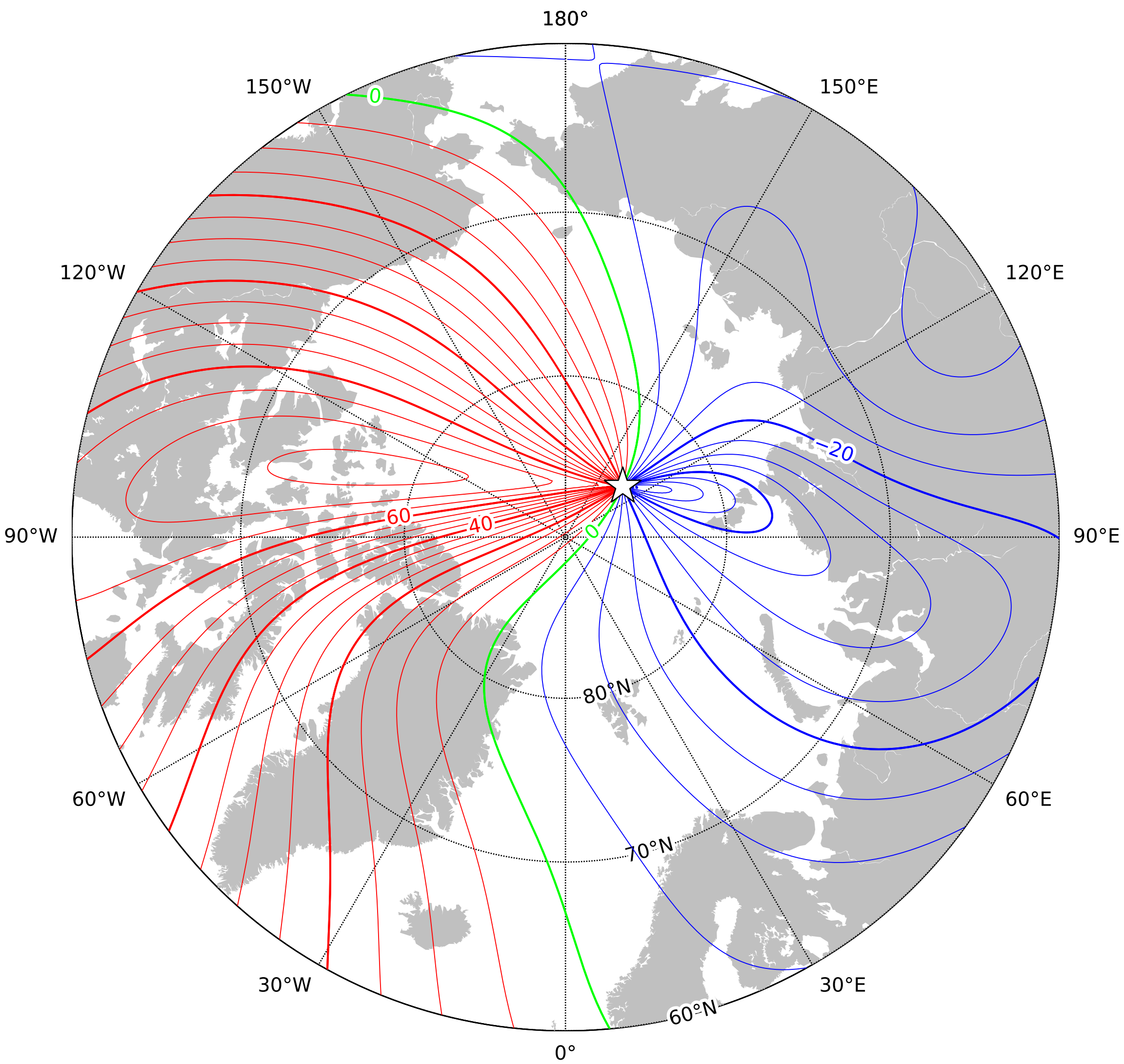
Annual rate of change of horizontal intensity in the region of the north pole at 2027.5 from the World Magnetic Model - High Resolution (WMMHR) 2025 (core component only). Red - positive change, blue - negative change, green - zero change. Contour interval is 5nT/year, white star is the location of a magnetic pole and the projection is Polar Stereographic. This is an example of an isoporic chart. British Geological Survey © UKRI 2024
