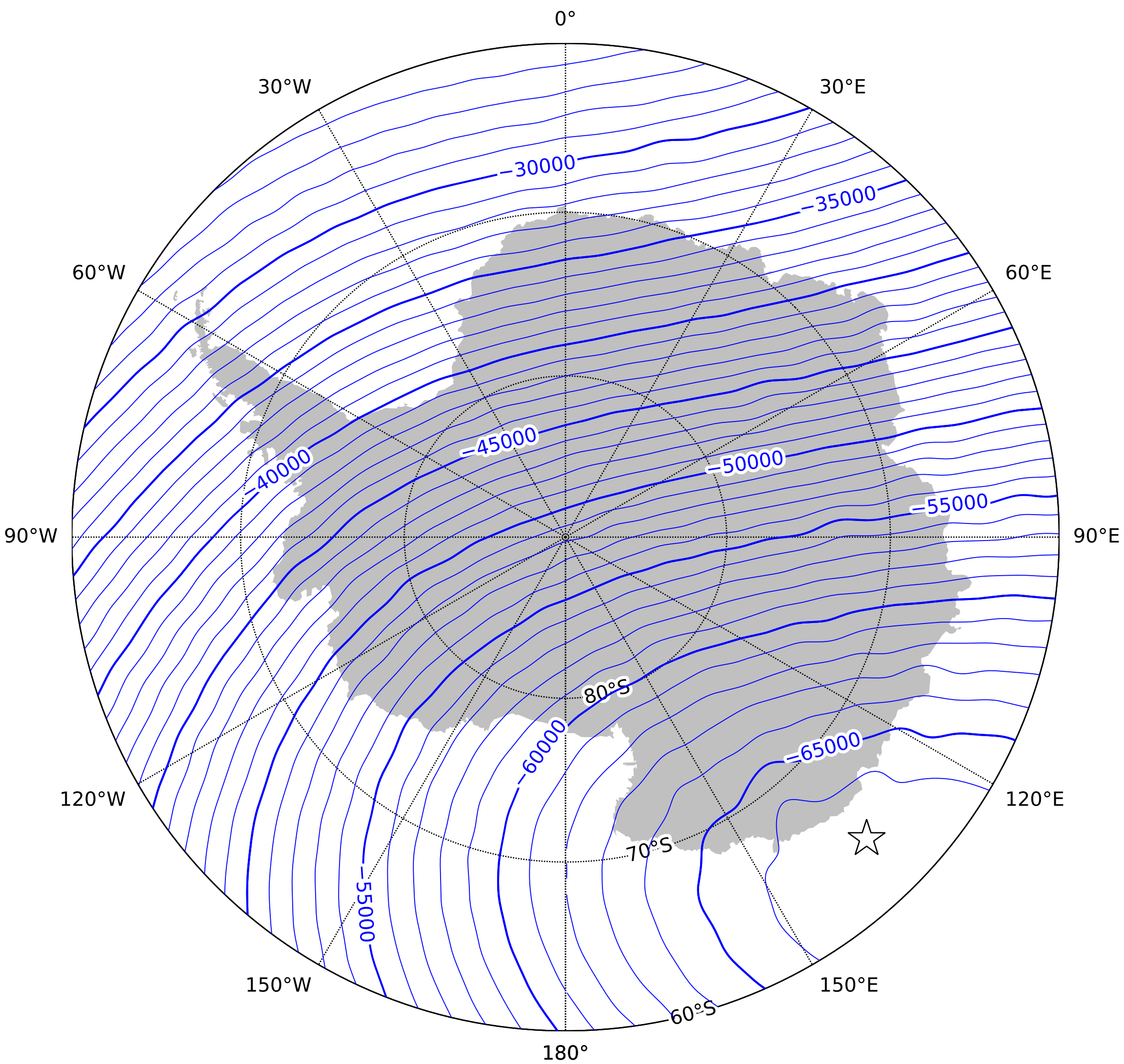
Downward component (Z) in the region of the south pole at 2025.0 from the World Magnetic Model - High Resolution (WMMHR) 2025. Red - positive (down), blue - negative (up), green - zero. Contour interval is 1000nT, white star is the location of a magnetic pole and the projection is Polar Stereographic. This is an example of an isodynamic chart.
